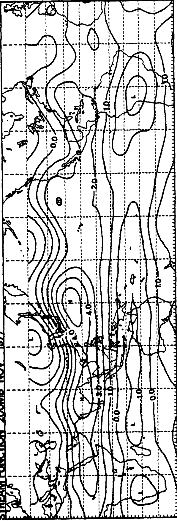
STREAM FUNCTION 200MB NOV 1977
